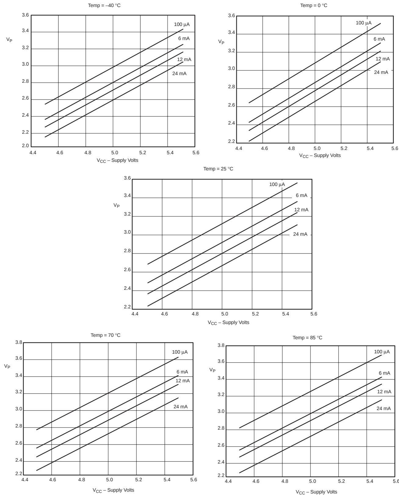
Figure 1. Typical characteristics
